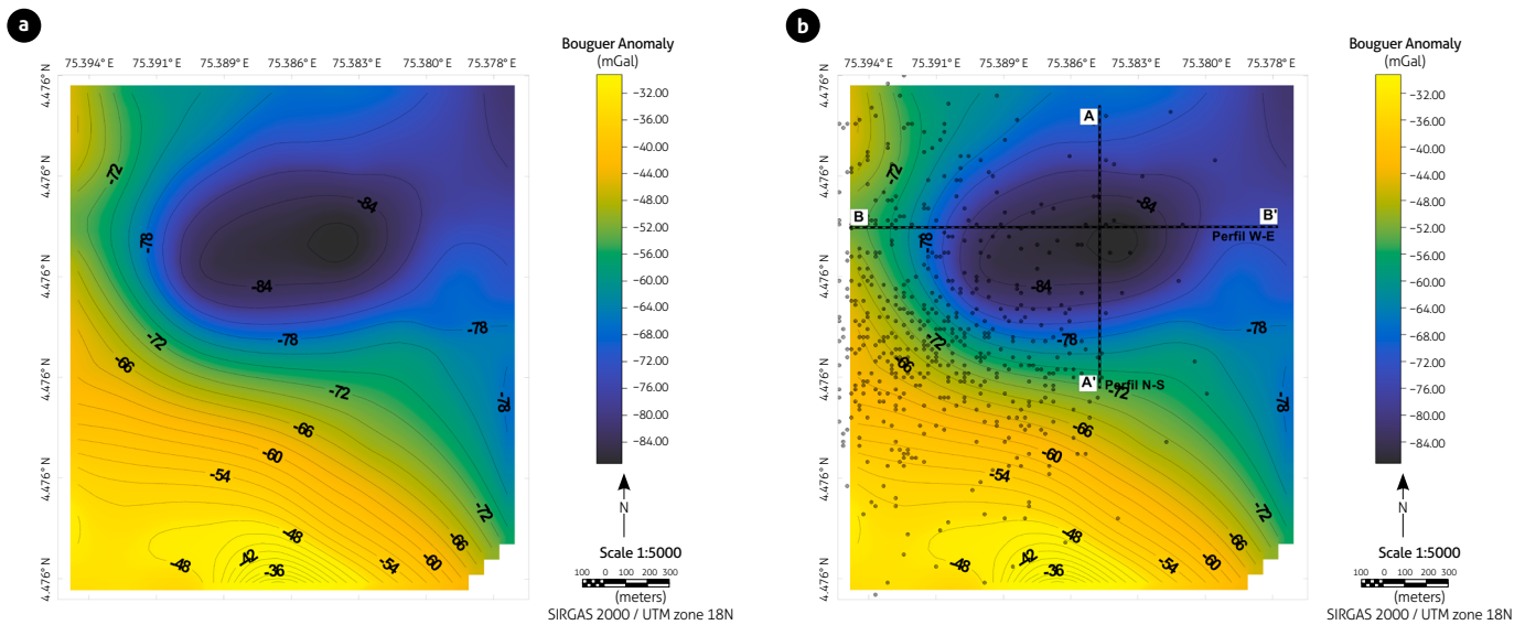
Figure 3. a) Bouguer map calculated using Equation 6 in the study area. b) Bouguer anomaly map, overlapped with the earthquakes shown by black dots, and the N-S and W-E transects for the depth models shown in Sections 3.3 and 4.2
