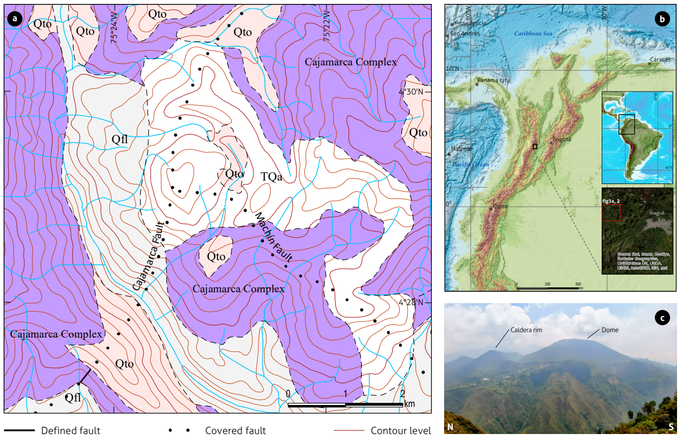
Figure 1. a) Geological map of the study area extracted from Geology Map 244 of the Servicio Geológico Colombiano (Mosquera et al., 1982), Machin fault from Méndez Fajury et al. (1996). b) Global and regional location of the Cerro Machin volcano in Colombia. c) N-S Panoramic view of the Cerro Machin volcano
