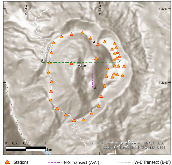
Figure 2. Map showing the contour level map showing the measurement stations throughout the volcano crater and the transects used on the 2D density models on Oasis
