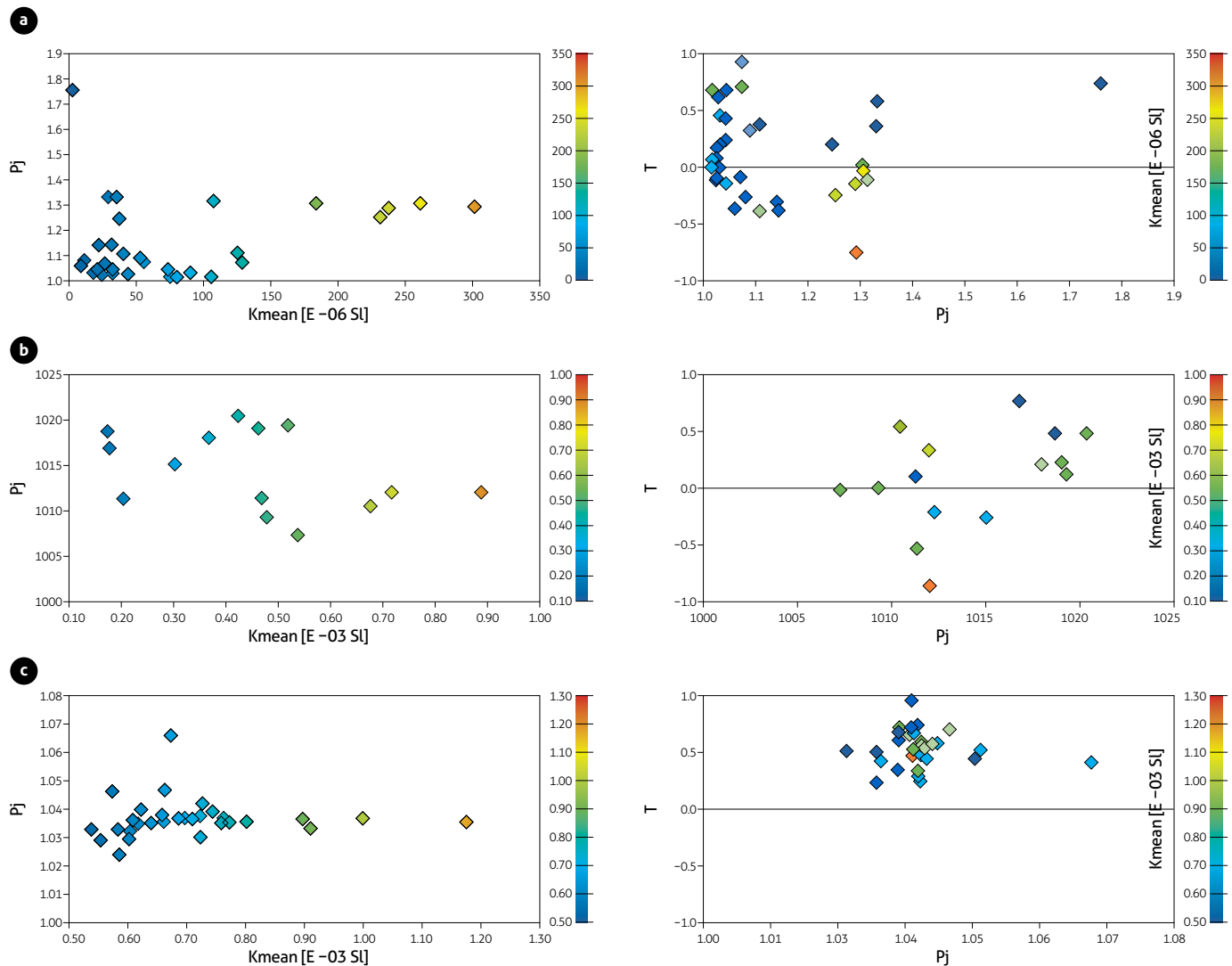
Figure 5. Mean susceptibility vs Corrected anisotropy shape factor and Jelinek diagram (Pj-T) of the deformed deposits at a) La Brizuela, b) Yarumalito, and c) La Caimana
