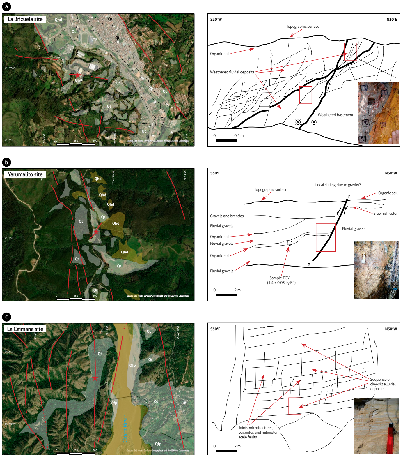
Figure 3. Selected sites for AMS analysis a) Faulted Pleistocene (?) alluvial deposit along the La Mosca satellite Fault at the La Brizuela site. b) Faulted Holocene soil along the San Jerónimo Fault at the Yarumalito site. c) Apparently undeformed Holocene deposits covering the Cauca West Fault close to Santa Fe de Antioquia town. Red stars mark the specific location of the AMS analysis while red lines are the local faults covered by Quaternary deposits (Qt = Terrace, Qfp = Flood plain, Qhd = Hillslope deposit)
