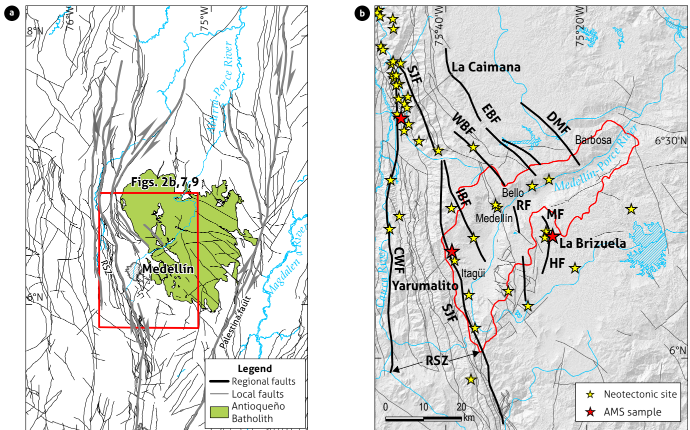
Figure 2. Detailed tectonic and geomorphic expression of the Central Cordillera controlling AV’s morphotectonic a) Main tectonic boundaries in the Northwestern Andes (black lines) and location of the study site between the RSZ, and the Antioqueño Batholith which is shown as green polygon in the center of the Central Cordillera (Gómez-Tapias et al., 2015). b) Active faults in the surroundings of the AV, named as SJF = San Jerónimo Fault, CWF = Cauca West Fault, IBF = Iguaná-Boquerón Fault, WBF = Western Belmira Fault, EBF = Eastern Belmira Fault, RF = Rodas Fault, DMF = Don Matias Fault, MF = La Mosca Fault, and HF = La Honda Fault. Along these faults several neotectonic sites have been reported previously (see Table 1), and three of them were selected for AMS analysis.
