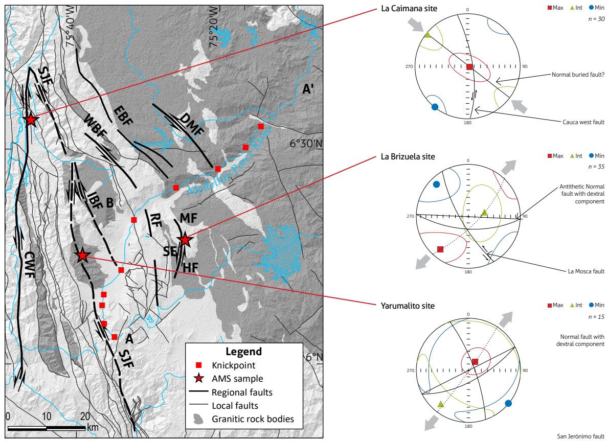
Figure 7. Comparison of magnetic fabric ellipsoid and structural datasets of active faults at La Caimana, La Brizuela, and Yarumalito sites, and a synthesis of the Riedel shear model indicating the occurrence of primary and secondary structures under a known strain field. Longitudinal river profile is marked from A to A'. SJF = San Jerónimo Fault, CWF = Cauca West Fault, IBF = Iguaná-Boquerón Fault, WBF = Western Belmira Fault, EBF = Eastern Belmira Fault, RF = Rodas Fault, DMF = Don Matias Fault, MF = La Mosca Fault, and HF = La Honda Fault. B = Baldías, SE = Santa Elena.
