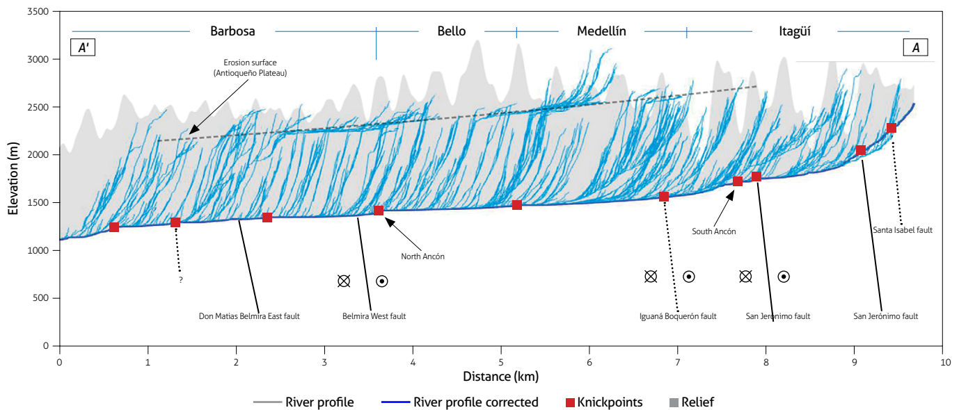
Figure 8. Longitudinal profile of the Medellín Porcía River indicating the spatial distribution for the four tectonic basins of the AV separated by local faults (Rendón, 2003)
