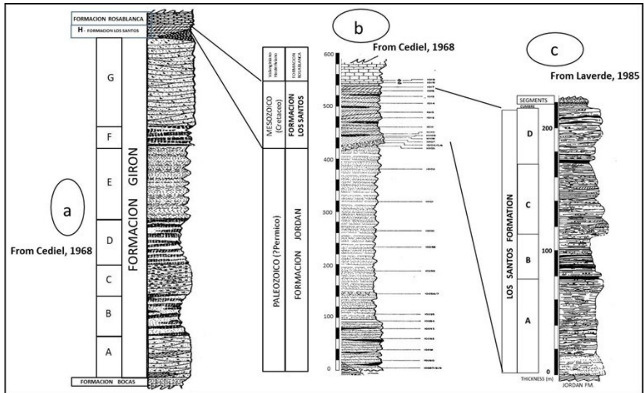
Figure 3. Stratigraphic columnar sections about the Giron and Los Santos formations. (a) Giron Group consisting of the Giron Formation in the type section of Lebrija river gorge and Los Santos Formation (after Cediél, 1968). (b) Stratigraphic column of the Jordan and Los Santos formations at the type locality for both units in the El Roto trail (Cediél, 1968). (c) Stratigraphic column of the Los Santos Formation in the type section of El Roto trail (from Laverde, 1985).
