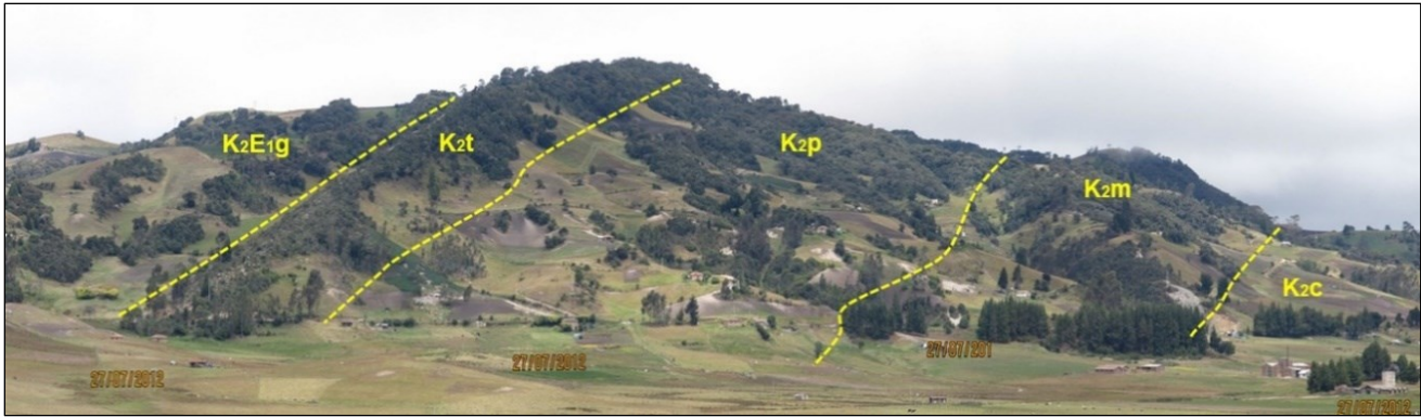
Figure 2. Characteristic geomorphology of the Guadalupe Group units in the study area. The Motavita (K2m) and Arenisca Tierna (K2t) formations show steep geofoms that alternate with valleys or depressions originated by the Conejo (K2c), Plaeners (K2p) and Guaduas (K2E1g) formations. View to the SW from the Quebrada Honda village in the municipality of Motavita (N= 1 115 657, E= 1 080 404, Z= 3 081, Azimuth= 215 °)
