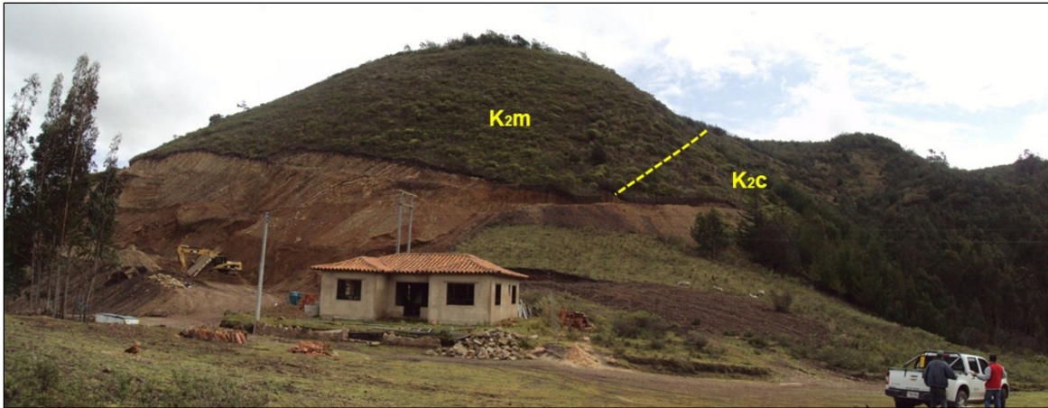
Figure 8. Approximate geological contact between the Conejo (K2c) and Motavita (K2m) formations
