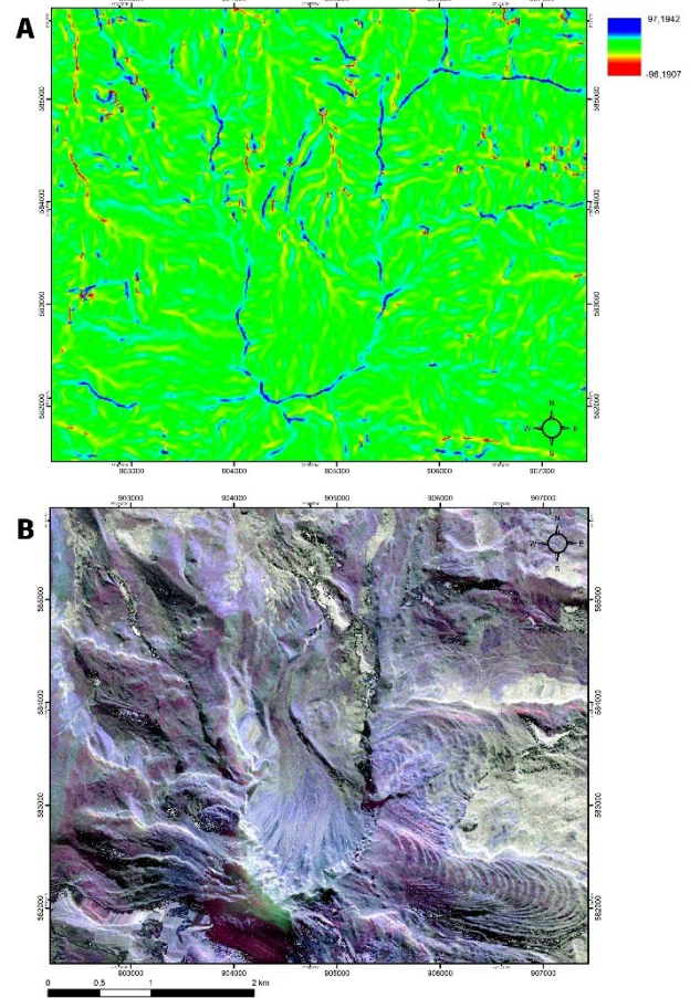
Figure 3. Convergence Index calculated for the area of interest. Values closer to 100 (blue tones) outline ridges, while values closer to -100 (red and yellow colors) highlight deep gullies. (B) UAVSAR mission L-band polarimetric SAR image of the area of interest with |HH-VV| , |HV| , and |HH+VV| as RGB channels. Modified from National Aeronautics and Space Administration (NASA) (2015).
