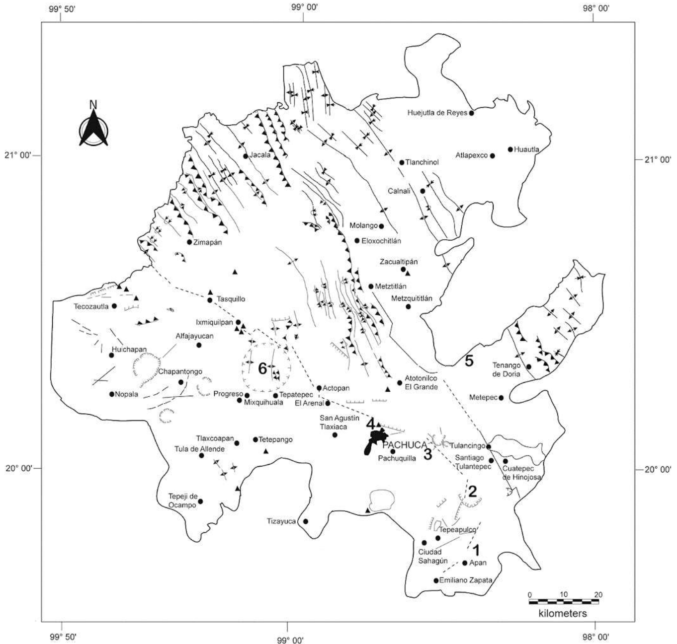
Figure 8. Simplified structural map of Hidalgo showing volcanic fields and sequences where the occurrence of adakitic rocks has been reported. 1 – Apan volcanic field, 2 – Chichicuautila-Tecomulco volcanic field, 3 – Epazoyucan - Singuilucan volcanic field, 4 – Sierra de Pachuca, 5 – Tulancingo north region, 6 – Panales caldera, this study.
