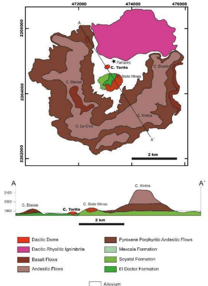
Figure 3. General geological map and cross section of the Panales caldera -named after the village of Panales. To the southwest of Panales, is located El Torito dome (modified from Barrera-Guerrero, 2009).
