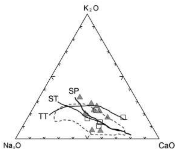
Figure 9. K 2 O-Na 2 O-CaO triangular diagram of representative rock analysis of the Panales caldera and nearby areas to the north, showing the trondhjemite (TT), sodic (ST), in comparison to the Sierra de Pachuca volcanic trends (SP). Discontinuous line represents the adakitic field. Squares represent volcanic rocks and solid triangles plutonic rocks.
